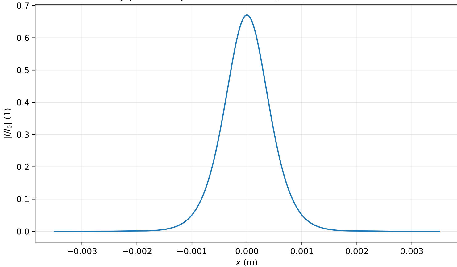
Intensity profile I(x, y = 0, z = 3.742m)/I_0 , P_{in}=0.7P_{cr} , artificial time
